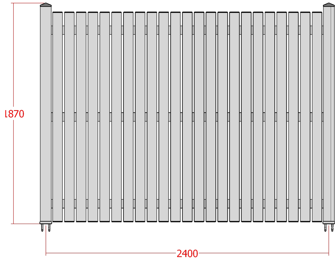
1800 H x 2400 W FENCE M01
